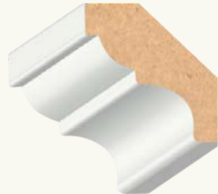
TCCRM-2 Dimensions 9/16 x 1-7/8
